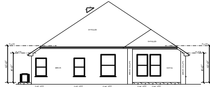
REAR ELEVATION SCALE: 1/4"=1'-0"
